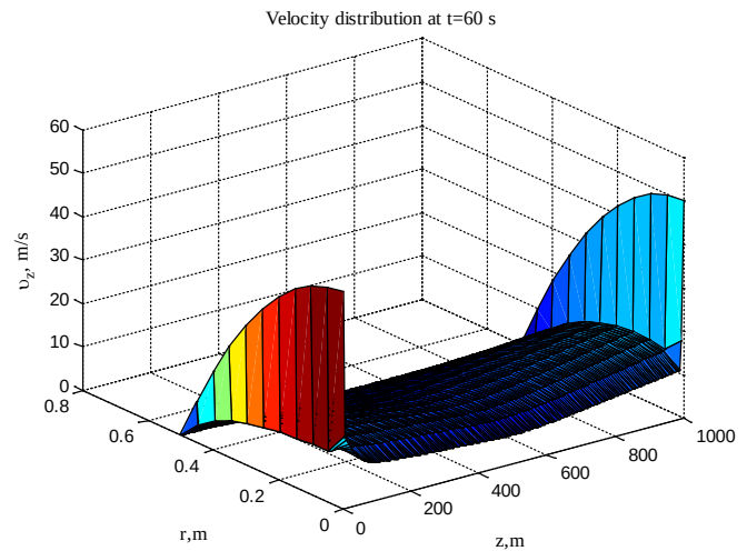
Fig. 1. The velocity v_z field
