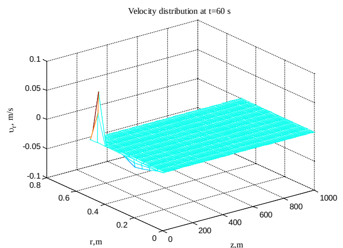
Fig. 3. The velocity v_r field
